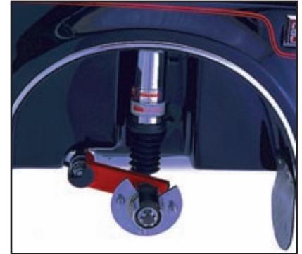
The fully adjustable air shock and internal coil spring with a trailing swing arm produces a totally independent suspension system.
